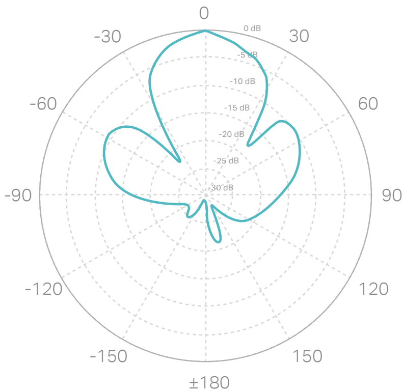
Horizontal Azimuth
