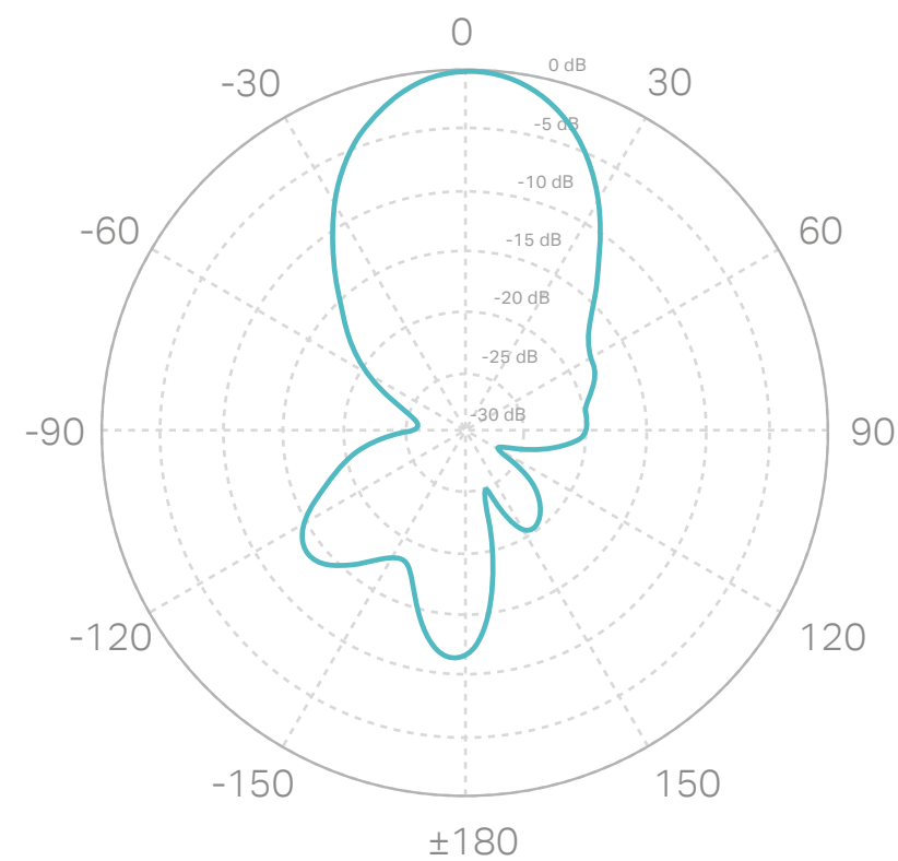
Vertical Elevation
