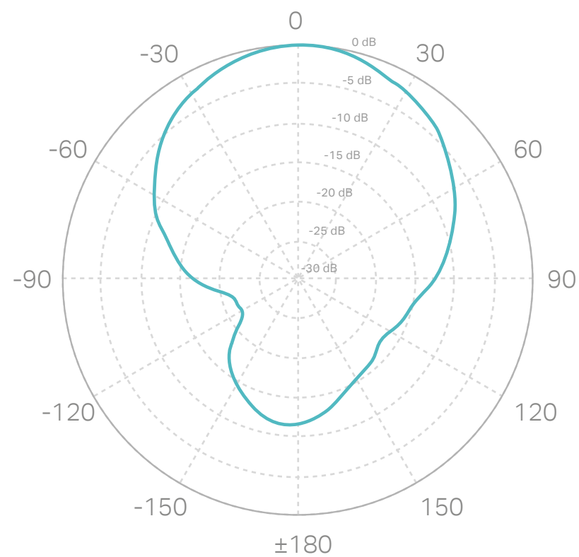
Vertical Azimuth
