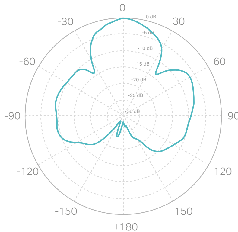
Horizontal Elevation
